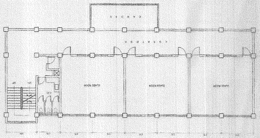
TYP. FLOOR PLAN
